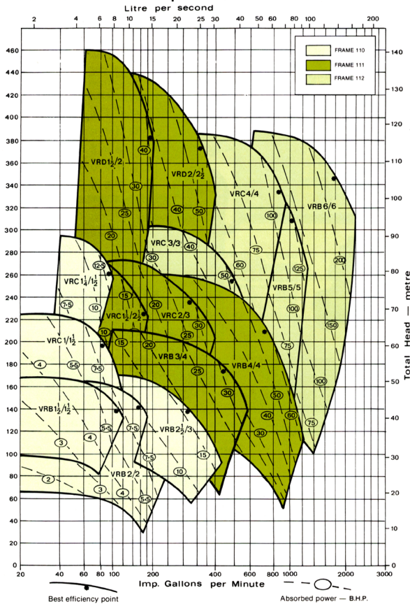
Performance at 2950 r.p.m.
